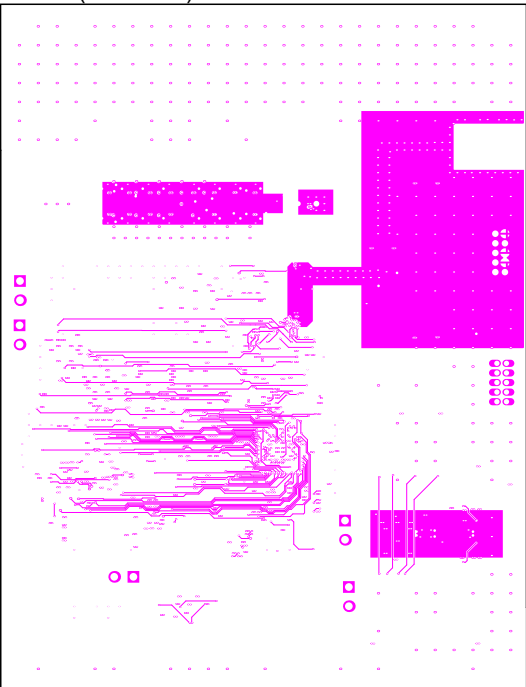
GND 3 (Scale 1:1)
