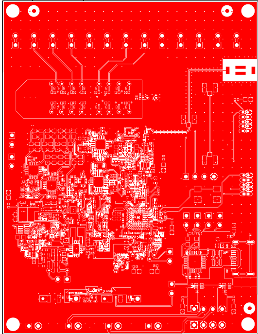
GND 2 (Scale 1:1)
